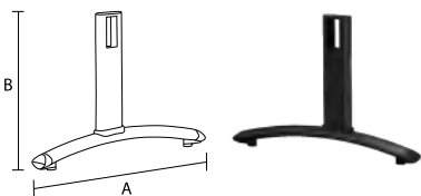
16 91gm-gamba mobile per panca con accessori 91gm-movable leg for bench with accessories
