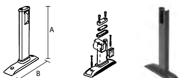
14 90gf-gamba fissa per panca con accessori 90gf-fixed leg for bench with accessories
