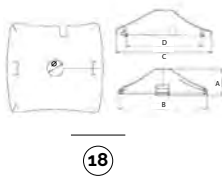
CPG plastic cover for swivel frame
