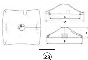
CPG plastic cover for swivel frame
