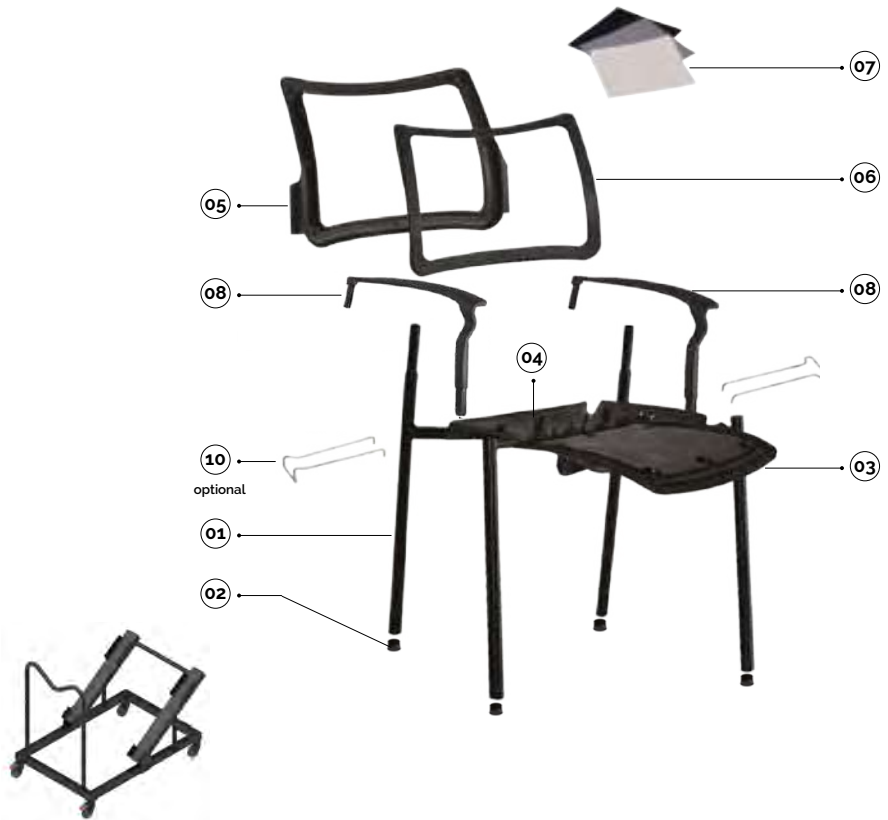
pinko-carrello portasedie con accessori pinko-trolley for chairs with accessories
